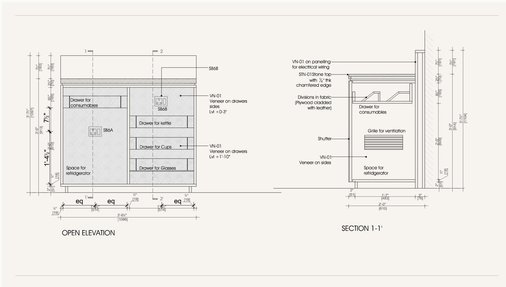
INTERIOR ELEVATIONS
